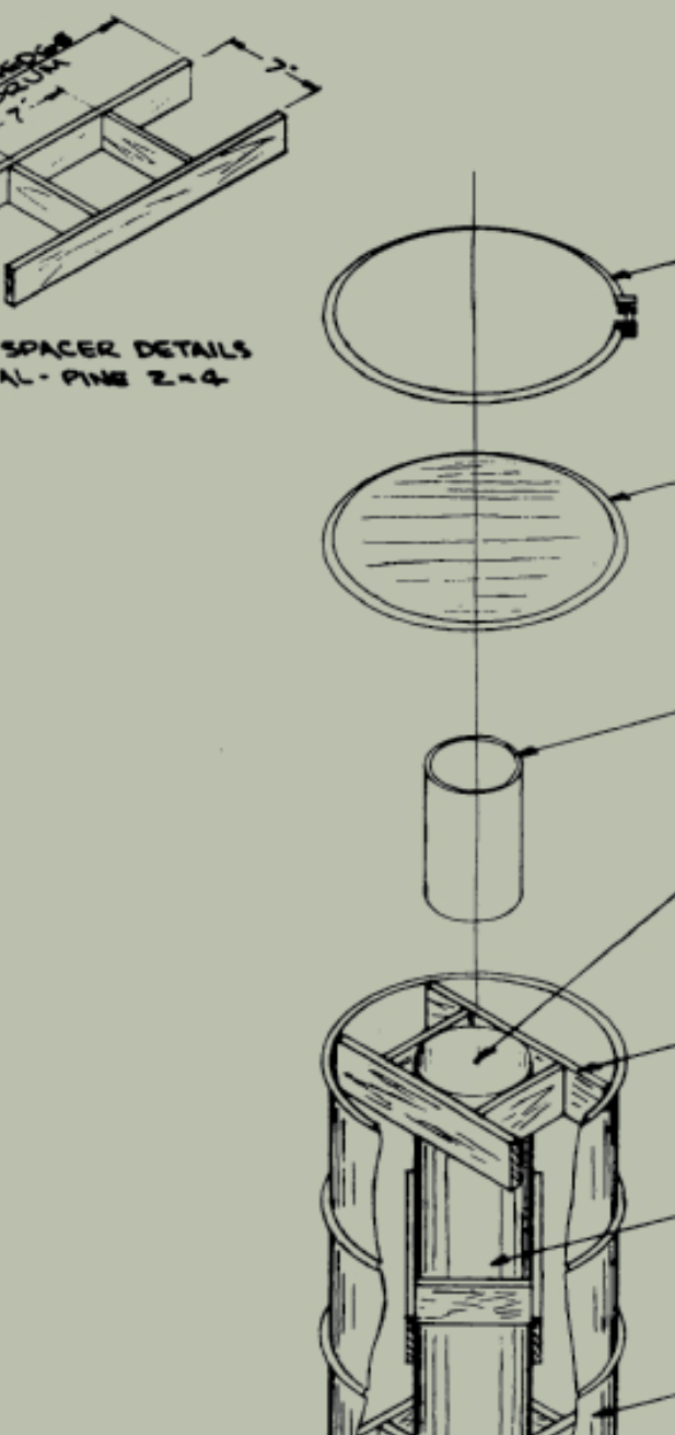
Diagram of a uranium scrap drum shipping container. From Nuclear Safety in Manufacturing Plants by James E. McLaughlin (New York: Health and Safety Laboratory, United States Atomic Energy Commission, 1959). From TRAIL collections.
